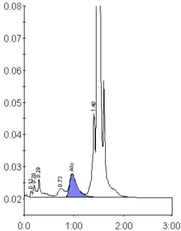
Peak table - ID: 10501699
